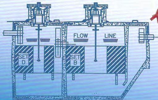
1500 gpd Plant
